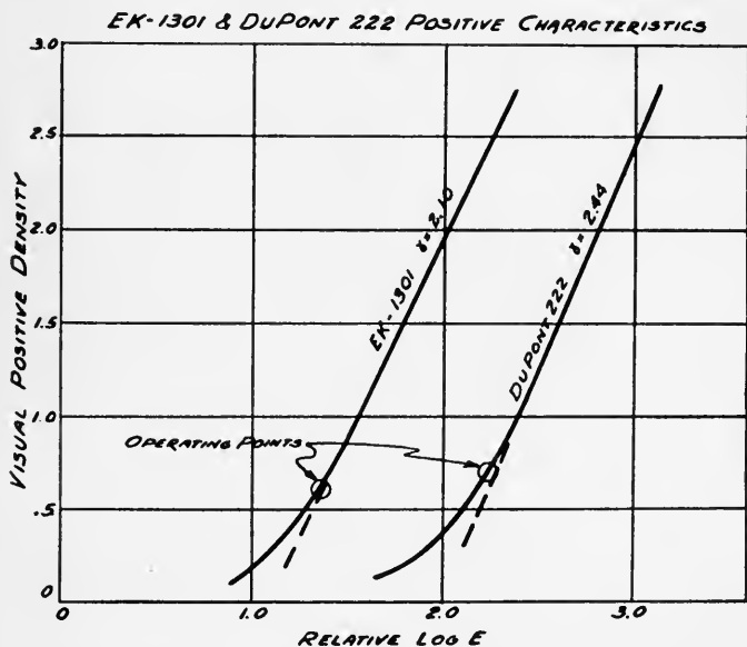
FIG. 1. I b sensitometric characteristics of Dupont 222 fine-grain and Ek-1301 positive emulsions in release positive developer; same development time.
